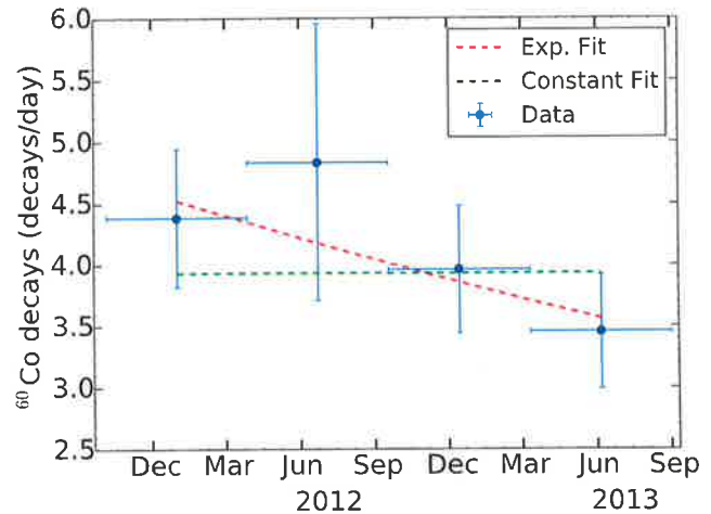
FIG. 5. (Color online) Behavior of ^{60}\text{Co} fitted decay rate in the TPC vessel vs time. The rate shown is counts integrated above 980 keV. (The full range used by the fit is 980–9800 keV, though the ^{60}\text{Co} PDF only extends to \sim 2.5 MeV). The vertical error bars on the points are those returned by the fit to the low-background data using the MIGRAD function of MINUIT [15,16]. Horizontal error bars show the size of the time bins. Two fits to the data are shown, including a constant and an exponential fit. The exponential fit produces a half-life of 1500 \pm 1100 days, consistent with the half-life of ^{60}\text{Co} . The \chi^2/\text{NDF} is 0.5/2 (2.35/3) for the exponential (constant) fit.
